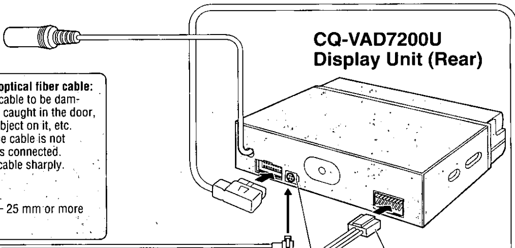
Optical Fiber Cable (CA-LRD60 : Option)
